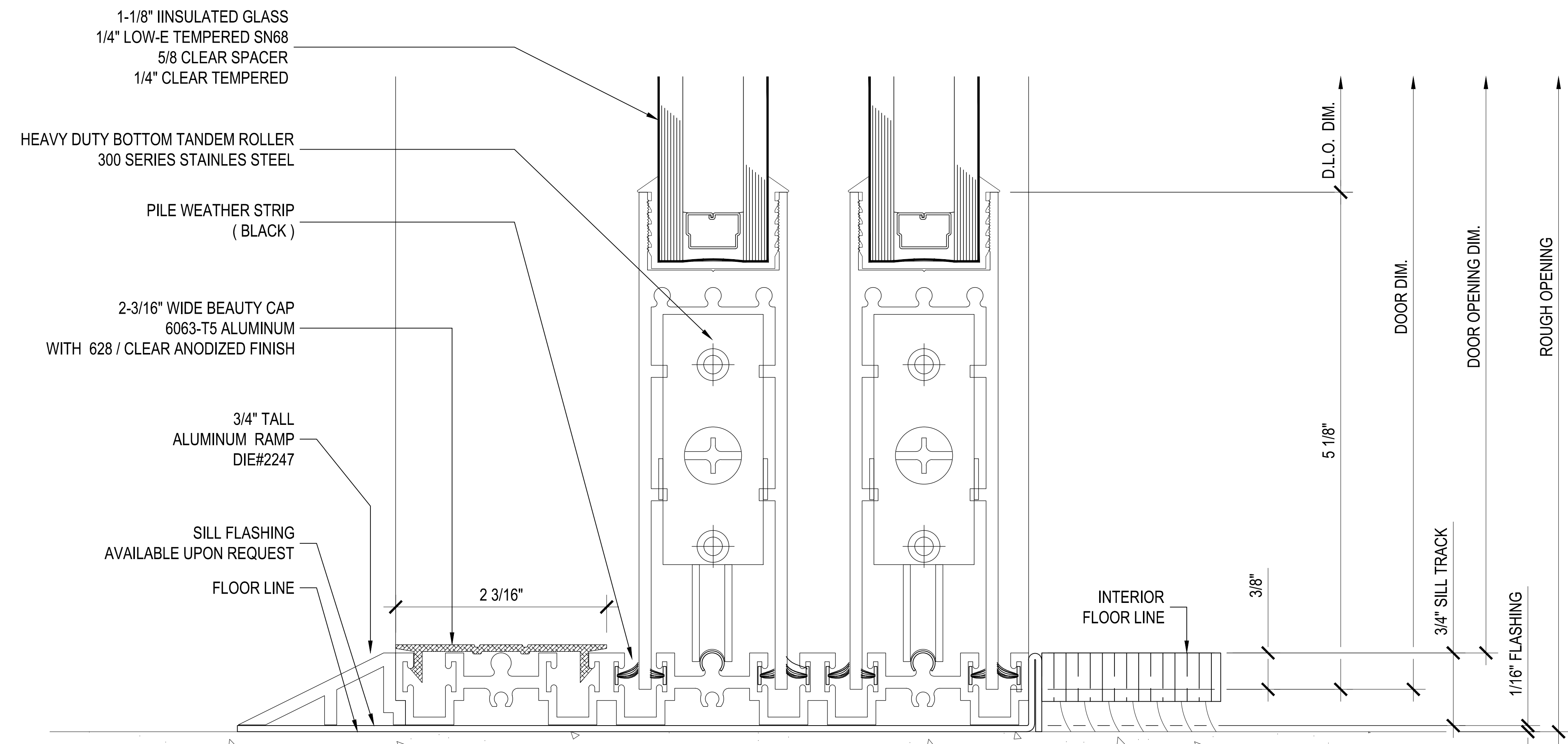
C Section @ (Slider) Max-Slider Sliding Glass Door (XXO)
