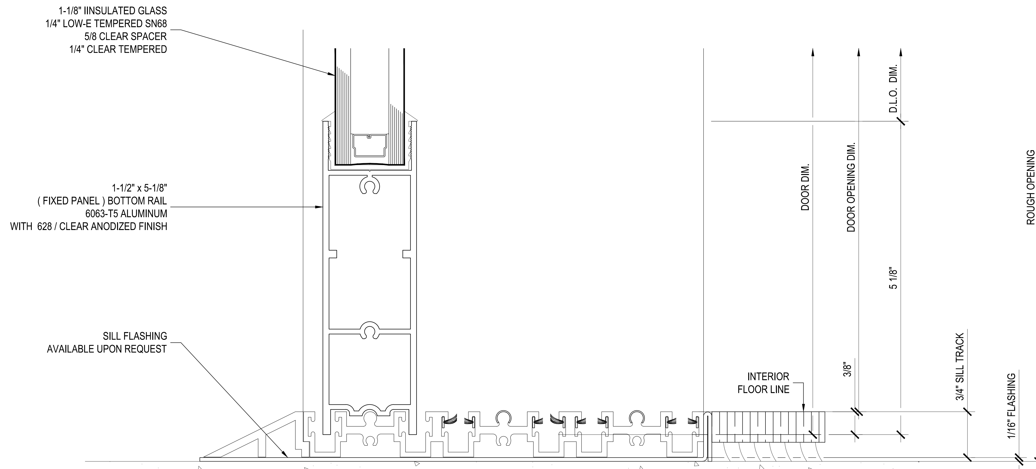
B Section @ (Fixed) Max-Slider Sliding Glass Door (XXO)
